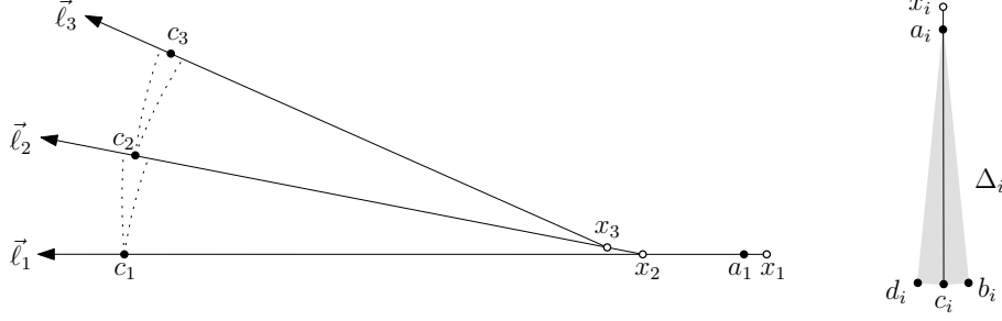
Figure 6: Left: The auxiliary point set P for k = 3 . Right: A long and skinny deltoid \Delta_i = (a_i, b_i, c_i, d_i) .
