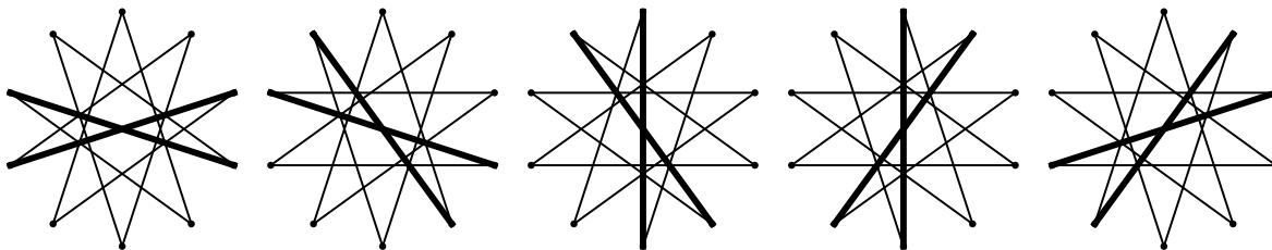
Figure 9: The 5 longest tours on the vertex set of a regular 10-gon. The two edges with span 5 are drawn with bold lines.
