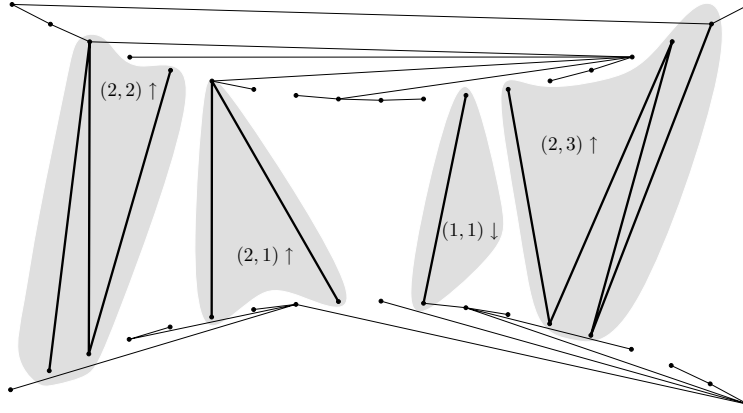
Figure 3: A double chain with lower and upper tree and four bridges.
