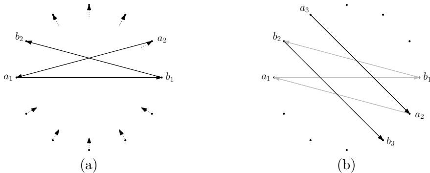
Figure 8: (a) A configuration that does not allow an extension to a longest tour, since the possible 5 “outgoing” edges have only 4 candidates to connect with. (b) A valid extension. The edges a_{i+1} \rightarrow a_i and b_i \rightarrow b_{i+1} form a pair of parallel edges.
