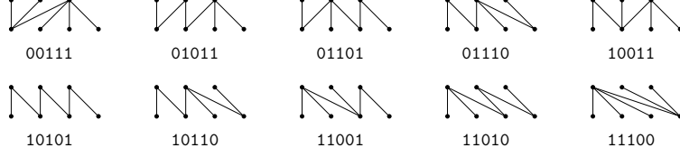
Figure 4: All B_{34} = 10 combinatorial types of (3, 4) -bridges. If an edge differs from its predecessor at the top we write a 0, otherwise a 1. We obtain a bijection between the bridges and sequences with three 1s and two 0s.
