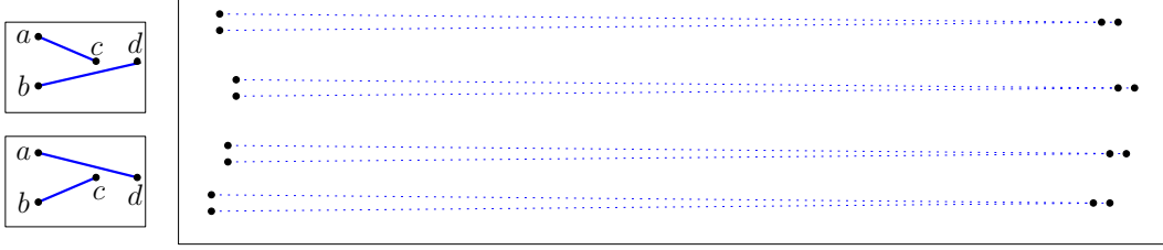
Figure 5: Left: Two possible maximum matchings for the point set S_4 = \{a, b, c, d\} . Right: A set of n = 16 points that admit 2^4 maximum non-crossing perfect matchings.
