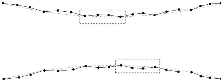
Figure 1: Two (flat) mutually visible copies of P^+(19, 2^6) with opposite orientations that form D(38, 2^{12}) . Two consecutive hull vertices of P^+(19, 2^6) with a reflex chain of two vertices in between are indicated in both the upper and the lower chain.
