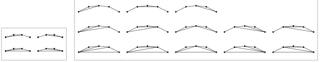
Figure 2: Left: Length reductions for the chains of D(n, 2^r) : two of type 1 and two of type 2. Right: Length reductions for D(n, 3^r) : three of type 1, five of type 2, and five of type 3.
